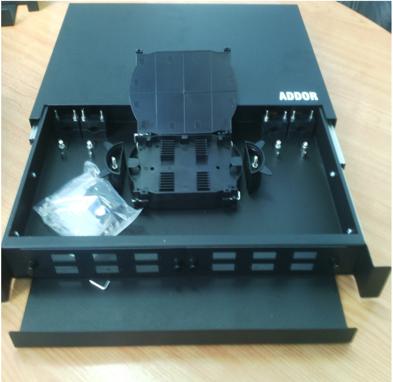
Ufibad Patch@ksh1748048Vot Drawable type with splicing tray for SC duplex adaptor -
